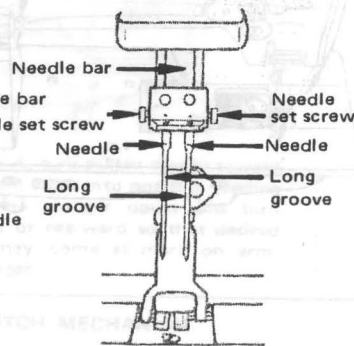
Fig. 9 (Two needle)
